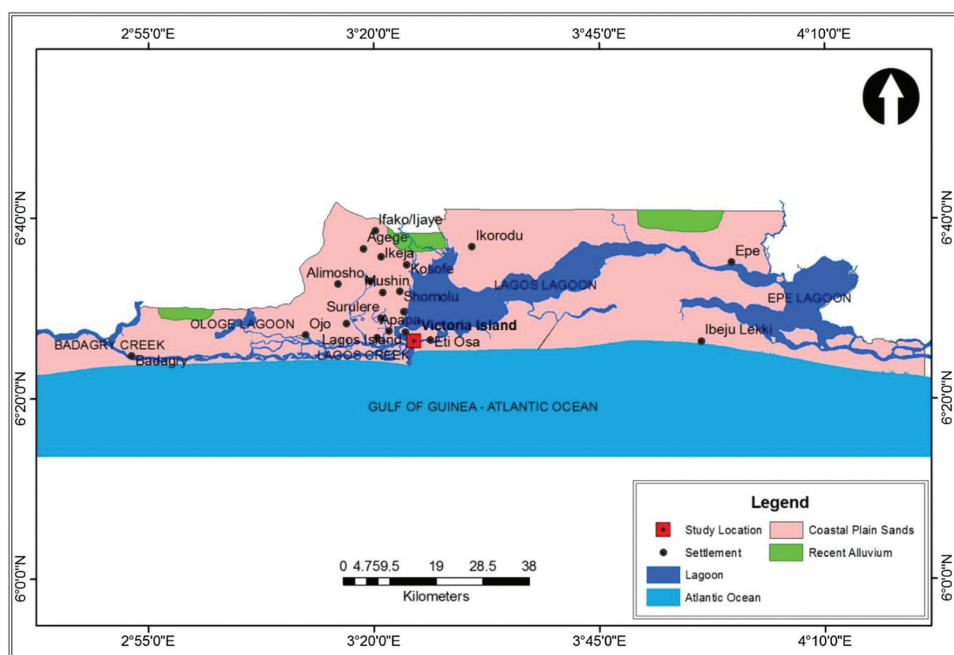
Figure 2. Geological map of Lagos State (culled from Olatinsu et al. 2018).
