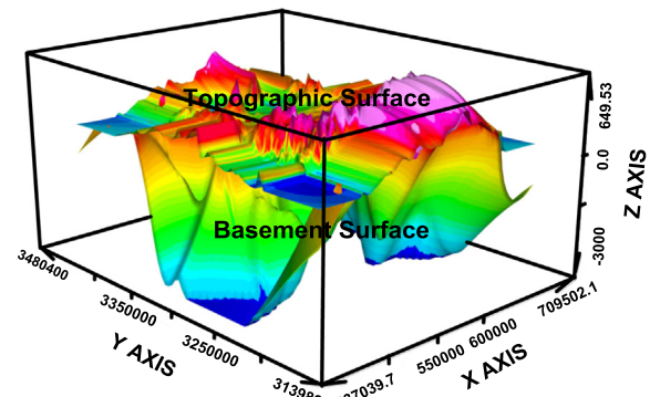
Fig. 14. Final three-dimensional (3-D) Magnetic modeling of the study area.
