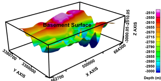
Fig. 17. 3-D gravity modeling of the basement surface of the study area.
