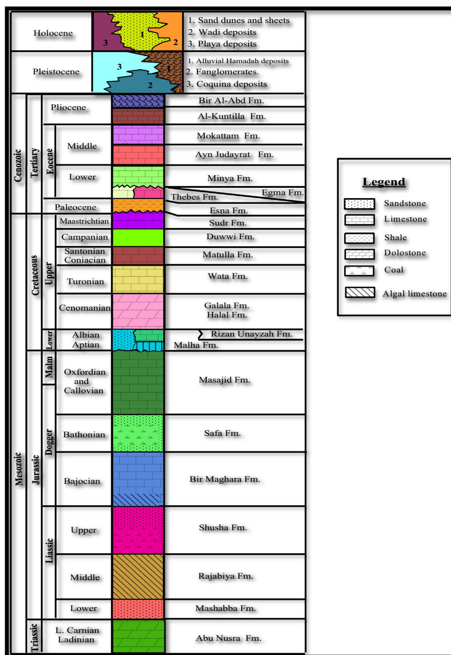
Fig. 3. Generalized stratigraphic column of north and central Sinai (compiled after EGSM, 1992, 1993 and 1994).
