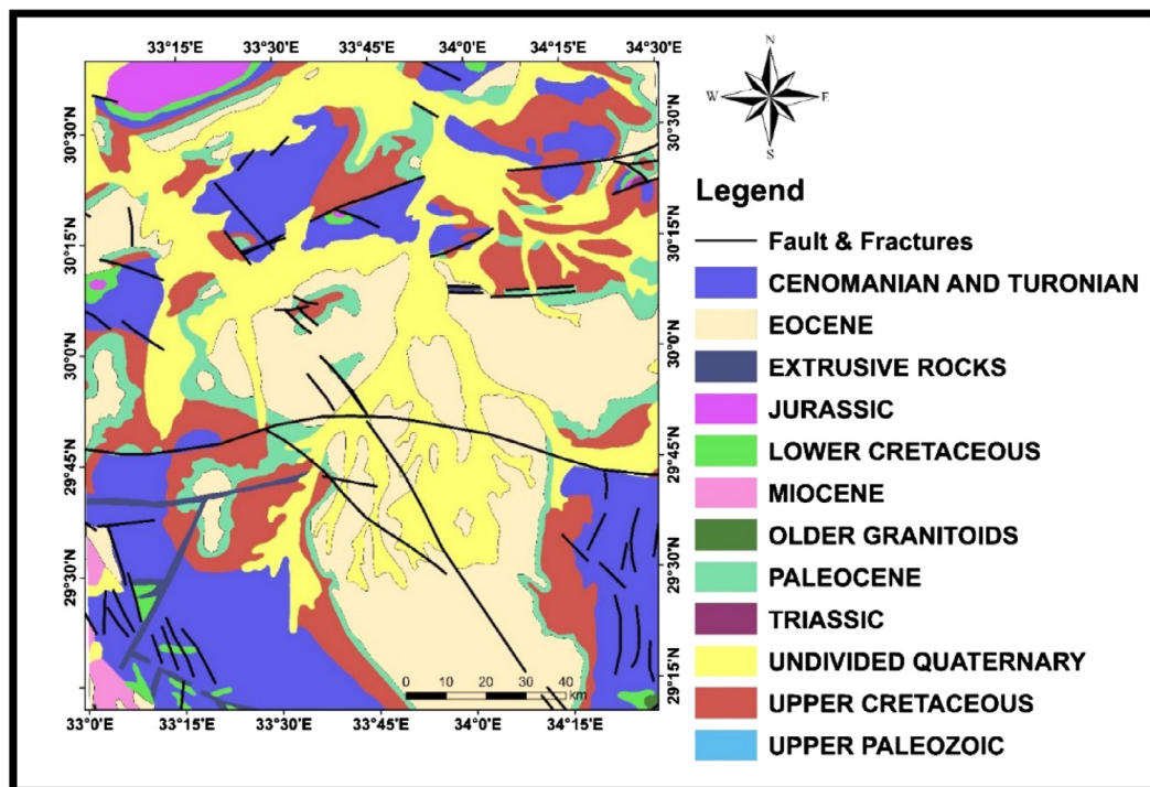
Fig. 2. Geologic map of the study area shows the main geological formations of the surface (Modified after EGSMA, 1981).
